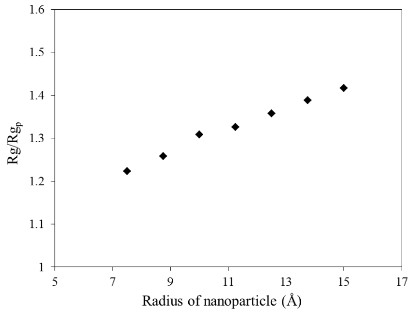
Figure 2.14. The ratio of the radius of gyration of polymer in presence of NP to that in absence of NP as a function of the radius of NP.
