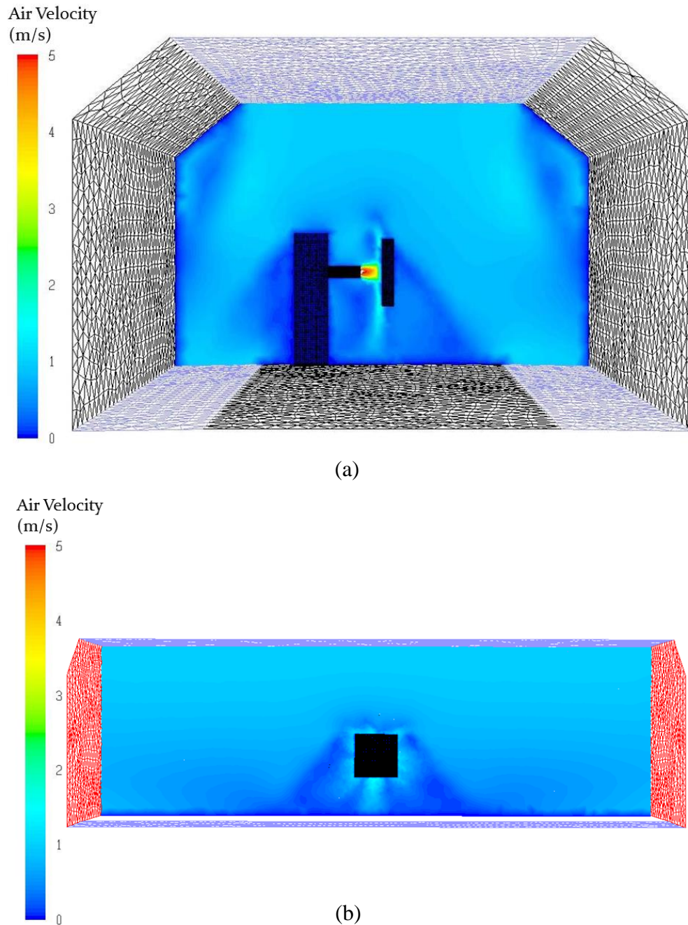
Figure 6.3. Air velocity contour (a) front view, (b) side view.
