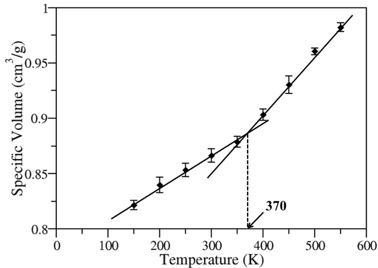
Figure 2.6. Determination of the glass transition temperature ( T_g ).
