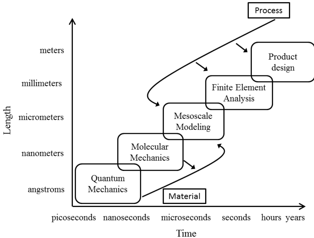
Figure 1.3. Multiscale modeling framework integrating top-down and bottom-up systems engineering approaches (McDowell and Olson, 2008).
